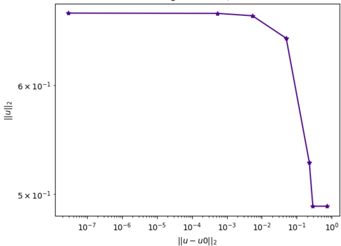
L-curve for TV regularization, \delta = 0.0001
