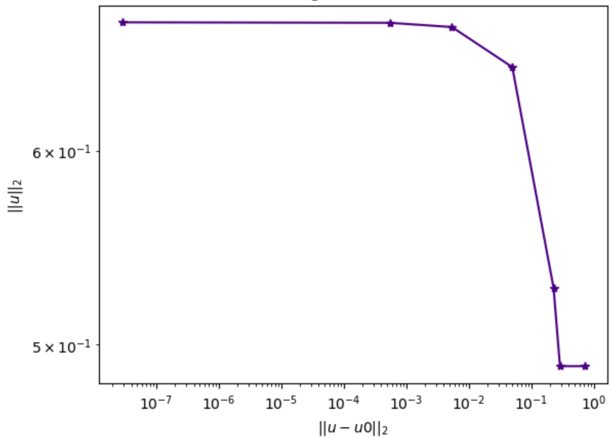
L-curve for TV regularization, \delta = 0.001
