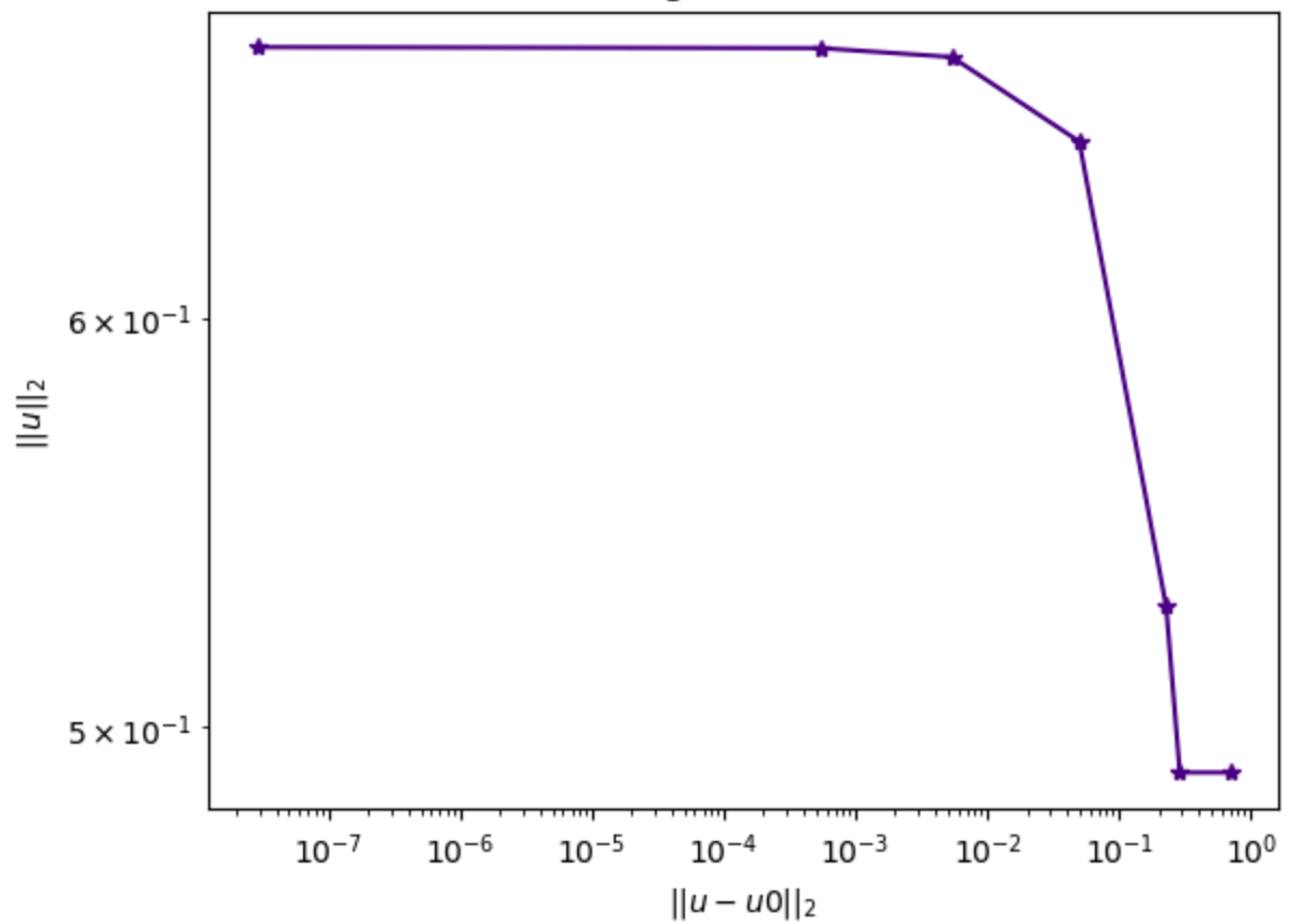
L-curve for TV regularization, \delta = 0.01
