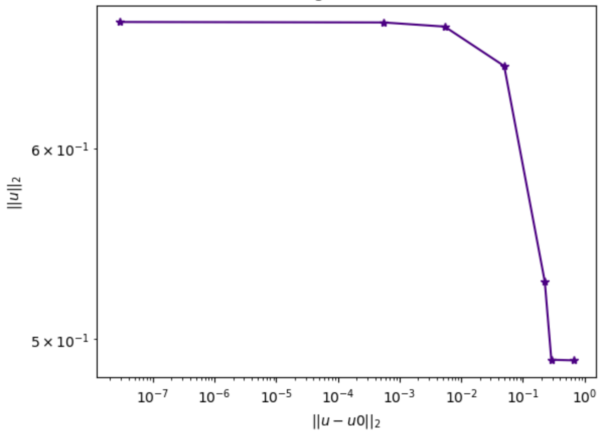
L-curve for TV regularization, \delta = 0.1
